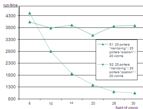
Figure 3: Simulation run-time with the strategies S_1 and S_2 for the third group
